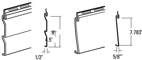
Double 4.5" Dutch Lap .042" thickness
