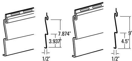
Double 4" Traditional .042" thickness
